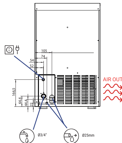
REAR VIEW VISTA POSTERIORE
