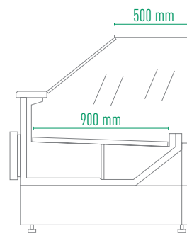
SAMA 125XL/150XL/190XL/250XL LATO / SIDE
